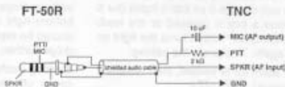
Detail of packet cable construction.
